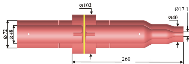
Figure 8: A cut away view of the cold window.
