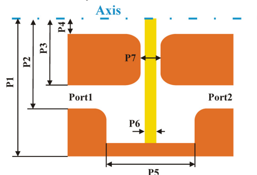
Figure 4: Window geometry parameters subject to optimisation
