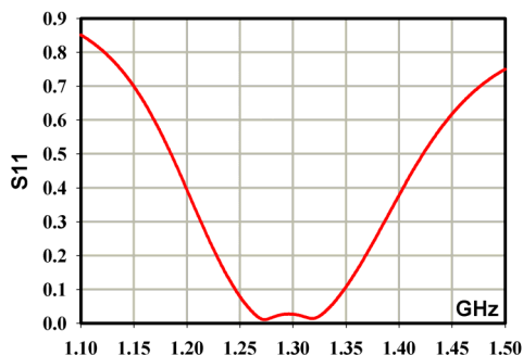
Figure 9: Frequency pass-band of cold window.
