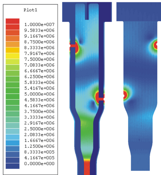
Figure 10: Distribution of magnetic field strength squared on the surface of part of the coupler.
