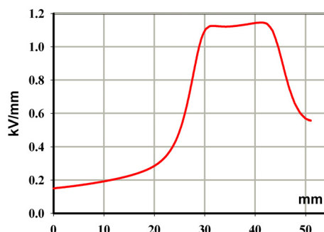
Figure 6: Electrical field distribution on the ceramic surface.
