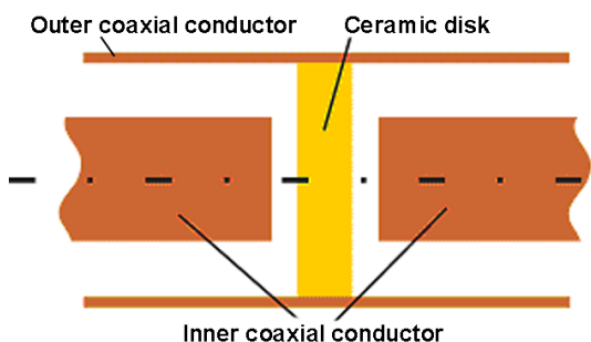
Figure 2: Conceptual sketch of the capacitive coupling for the rf window.
