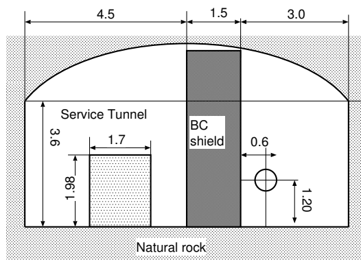
Figure 3: Cross section of Electron driver and Positron booster section. Tunnel is dug in the natural rock and the size is 9 m in width, 3.6 m in height. The height doesn't include the roof area.
