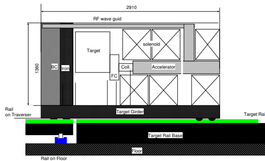
Figure 7: Vertical cross section of the target module moving from the target mount to the traverser. The target module contains not only the target, but also FC (Flux Concentrator magnet), the first accelerator tube, solenoid magnets, and front shields with BC and iron plate.
