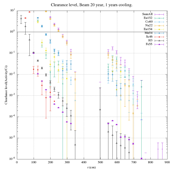
Figure 11: Clearance level of various elements and sum of them, as a function of the distance from the accelerator (target). The sum is below the clearance level at the natural rock, more than 500 cm from the axis.
