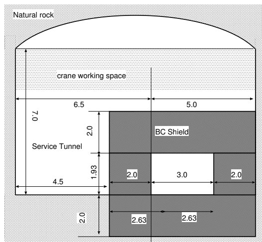
Figure 4: Cross section of ECS section. The accelerator tunnel is surrounded by 2 m BC shield to prevent the radio activity of the natural rock.
