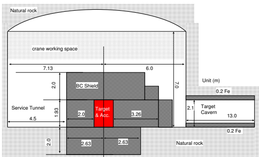
Figure 6: Cross sectional view of the target section. The center red square shows the target module. The module is surrounded by 2 m thick BC shield, not only the horizontal direction, but also vertical direction. Above the shield, working space for the crane is prepared. The size of the cavern is shrink in the figure.
