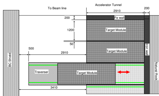
Figure 8: The horizontal view of the cavern. Target storage area is surrounded by iron plates for the radiation shield.
