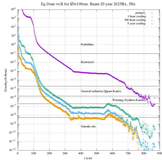
Figure 10: Radiation level after 20 years operation with various cooling time. Purple cross is just after the operation, x is 1 hour later, star is 100 hours later, and open box is 5 years later. The areas divided by horizontal lines show the category of radiation safety. From the top to bottom, the areas correspond to the forbidden area, restricted area, general radiation area, warning area, general area, and outside of the site.
