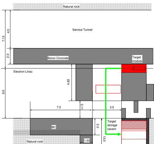
Figure 5: Horizontal view of the upstream part of the target section.
