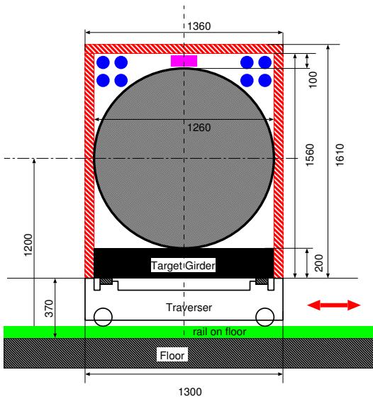
Figure 9: Front view of the target module on traverser. The module is surrounded by 5 cm iron shield. The 8 circles and one square on top of the shield show the joints and RF waveguide.
