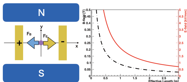
Figure 3: (left) The conceptual figure of Wien-filter. (right) The relation of electric and magnetic field and effective length.
