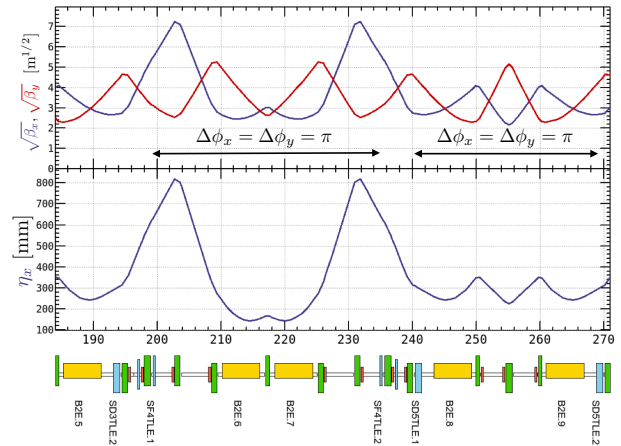
Figure 3: Design beam optics of the SuperKEKB arc section.
