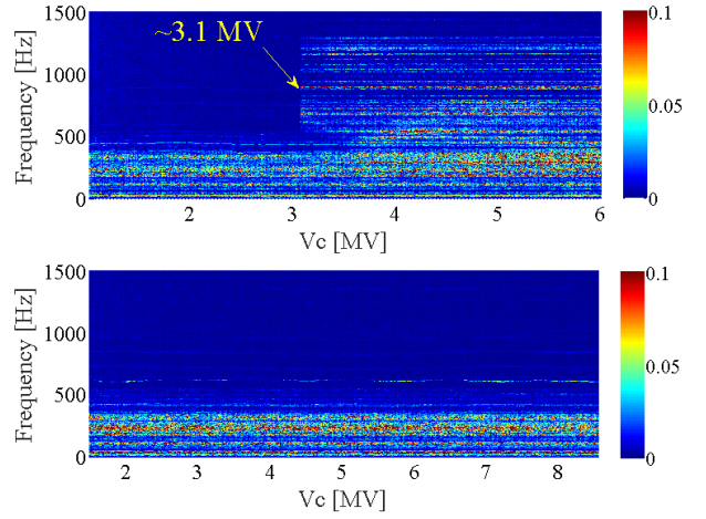
Figure 4: Field-detuning maps of ML1 (upper) and ML2 (lower) cavity. The color in the figure presents the intensity of the microphonics detuning.
