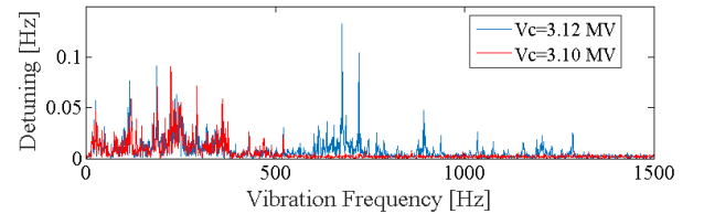
Figure 5: Microphonics spectrum comparison under the cavity field near the onset V_c .
