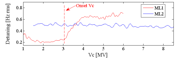
Figure 6: RMS detuning of the ML cavities as a function of V_c .
