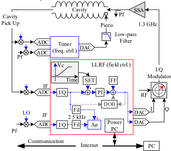
Figure 3: Schematic of the digital LLRF system and frequency tuner system of the cERL ML cavity.
