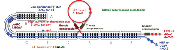
Figure 1: Schematic layout of the SuperKEKB injector linac.
