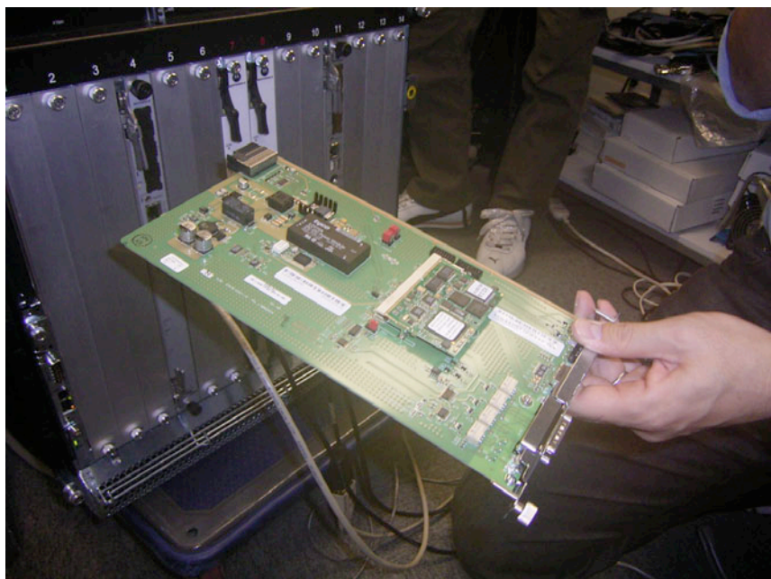
Redundant shelf manager units
