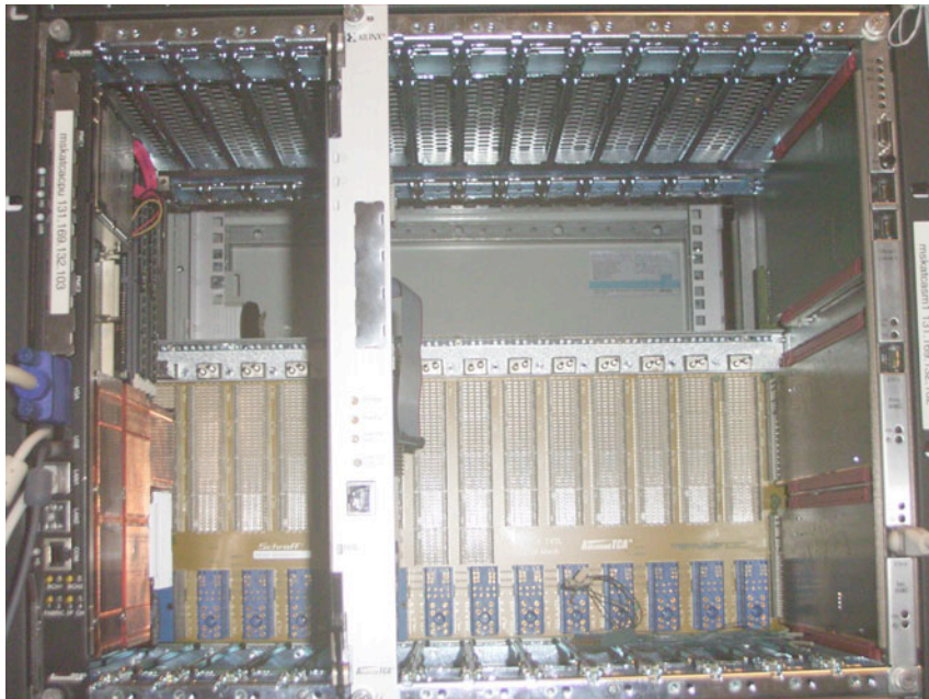
ATCA backplane
