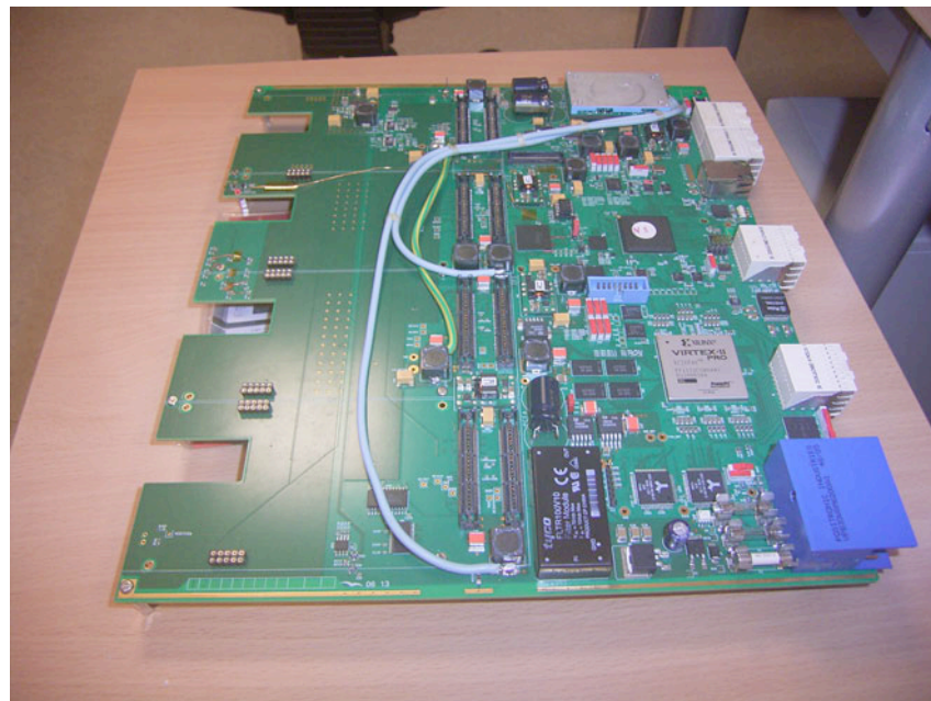
Carrier board for 4/8 AMCs
