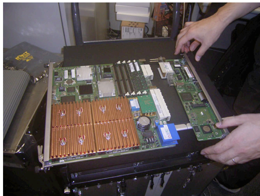
Redundant cpu と transition card
